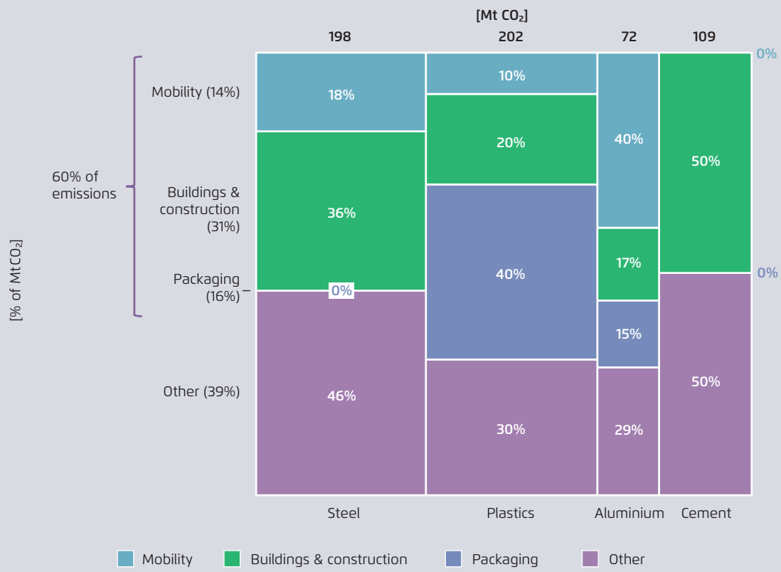
Emissions per material and value chain, EU % of MtCO 2 from materials used, 2019 (out of total)
