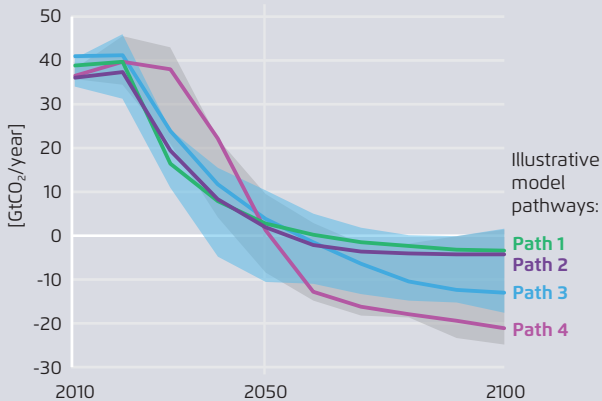
Negative emissions in various 1.5°C compatible IPCC scenarios
