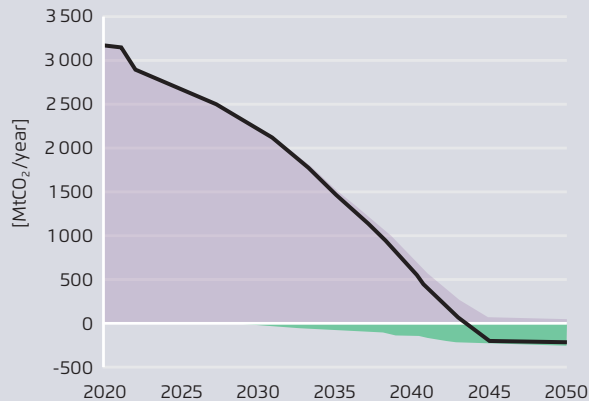
Negative emissions by steel sector in Technology Mix scenario
